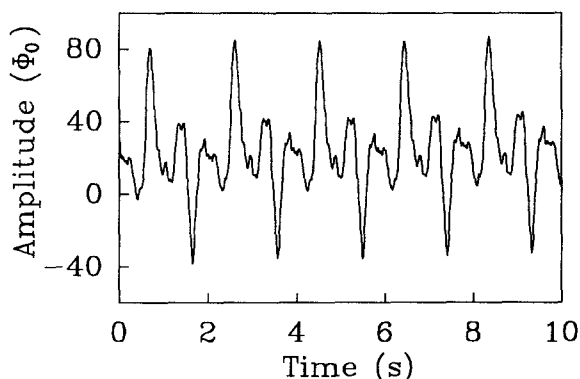
Figure 1. Difference between the number of flux lines trapped on the two hemispheres of the sample. The hemispheres are defined by the rotation of the sample at 0.5 Hz with respect to a fixed pick-up loop.
